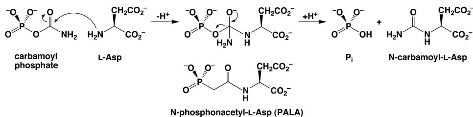
Figure 6 Aspartate transcarbamoylase (ATCase) catalyzes the condensation of carbamoyl phosphate with L-aspartate to yield N -carbamoyl-L-aspartate plus inorganic phosphate ( \text{P}_i ). The bisubstrate analog N -phosphonacetyl-L-aspartate (PALA) mimics structural features of both substrates and is a potent ATCase inhibitor. The binding of PALA reveals key intermolecular and intramolecular interactions that suggest a catalytic function for the phosphate group (Figure 7).
